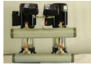
Vertical double pressure group with alternation and electronic pressure switch
